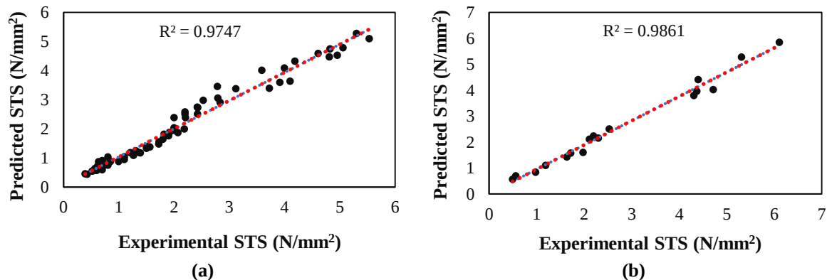
Fig. 9. Split tensile strength prediction for: a) Training; and b) Testing
