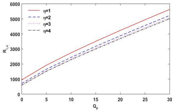
Fig 5a: Result of Q_F on R_{I,c} for diverse values of Casson constraint \eta for type (1) both boundaries isothermals.
