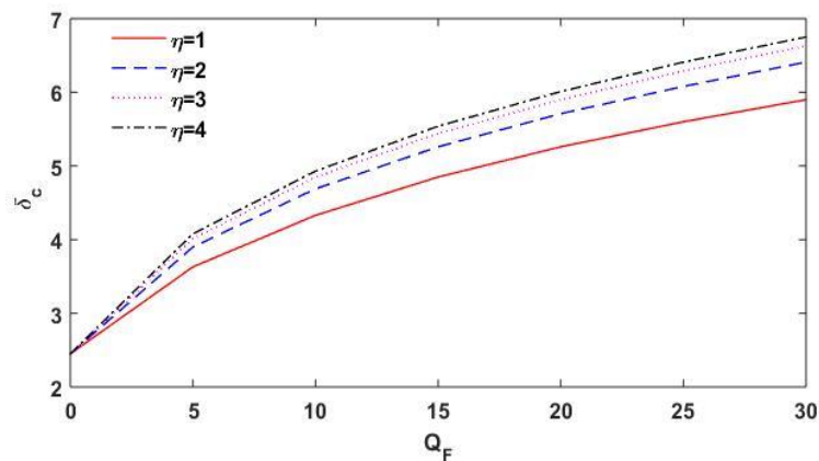
Fig 6b: Result of Q_F on \delta_c for diverse values of Casson constraint \eta for type (II) lower insulated and higher isothermal boundaries.
