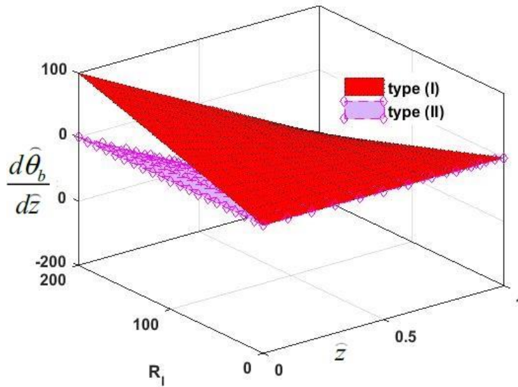
Fig. 2: Effect of internal Rayleigh number R_I on the distribution of basic temperature gradient \frac{d\hat{\theta}_b}{dz} .
