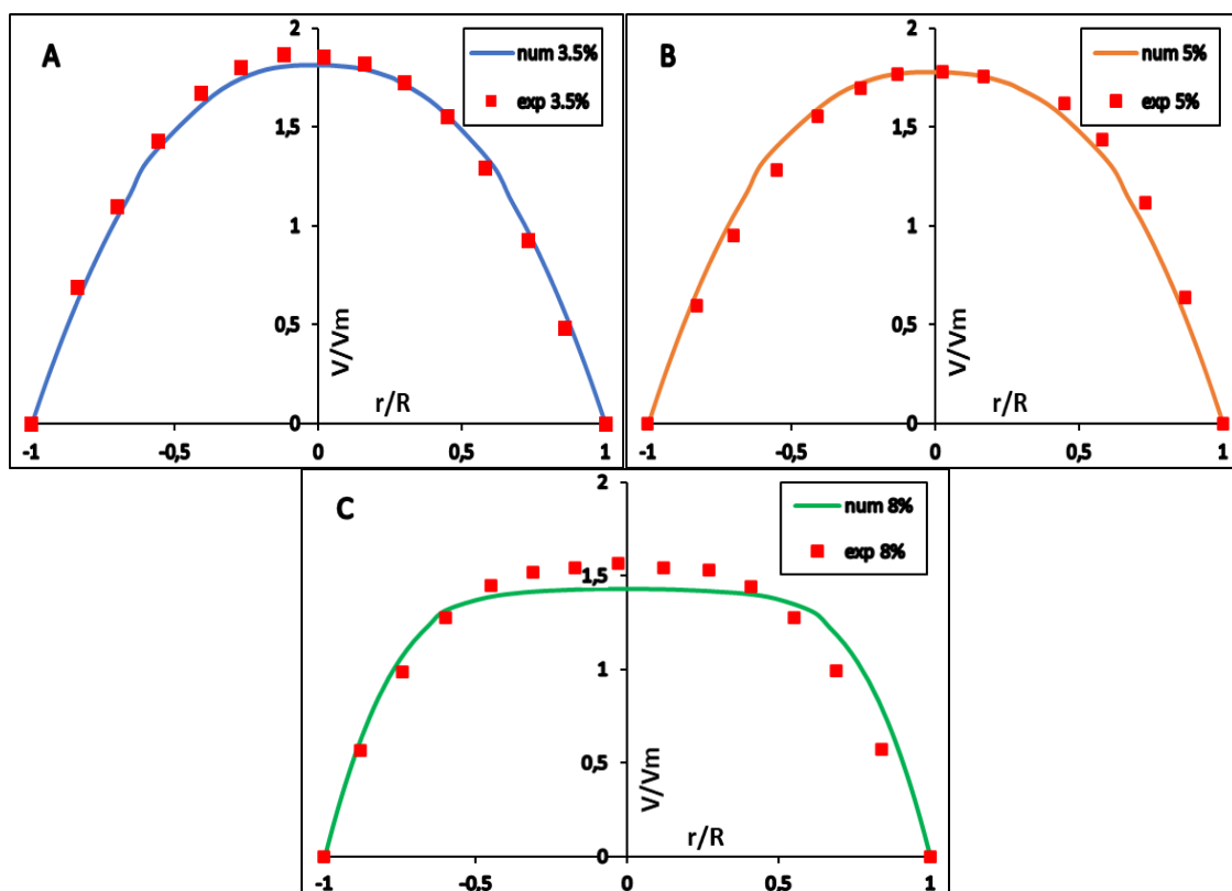
Fig. 7. Comparison of the numerical and experimental dimensionless velocity profiles for the three values of the index n , A: n=0.79 , B: n=0.68 and C: n=0.59
