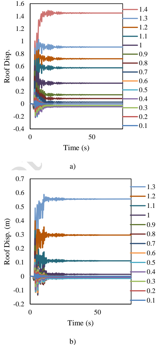
Fig.4. Roof horizontal displacement: a) ten-story building, b) six-story building
