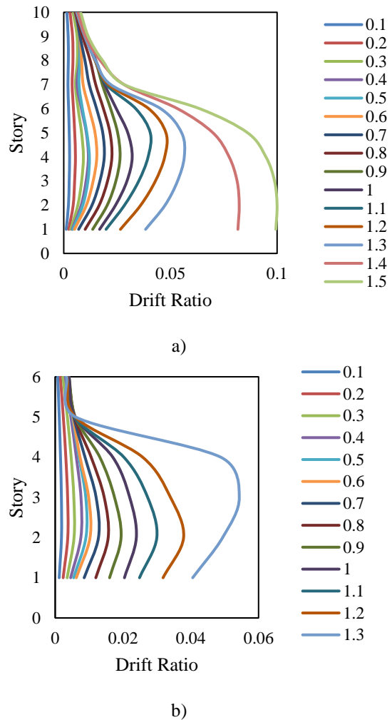
Fig.6. The maximum drift curve of the structure: a) ten-story building, b) six-story building
