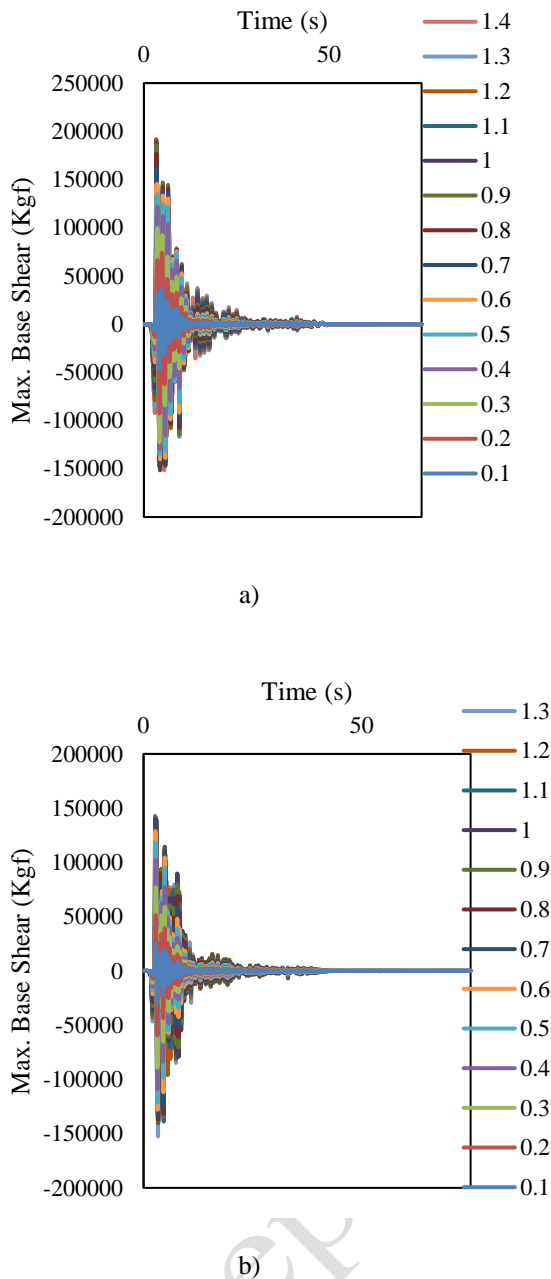
Fig.5. Time-history curve of the base shear in the structure: a) ten-story building, b) six-story building
