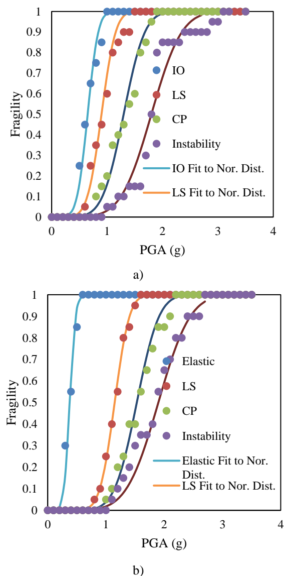
Fig.15. Fragility curve of the ten-story structure with: a) drift method, b) energy method
