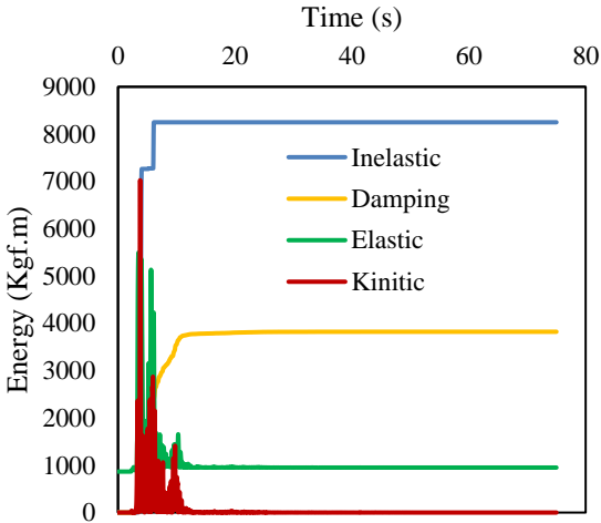
Fig.8. Time-history curve of the internal energy in the six-story building under Loma record with PGA=0.6g
