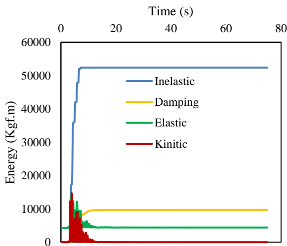
Fig.10. Time-history curve of the internal energy in the ten-story building under Loma record with PGA=0.7g
