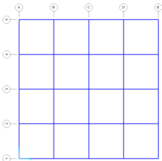
Fig.1. Structural Plan
