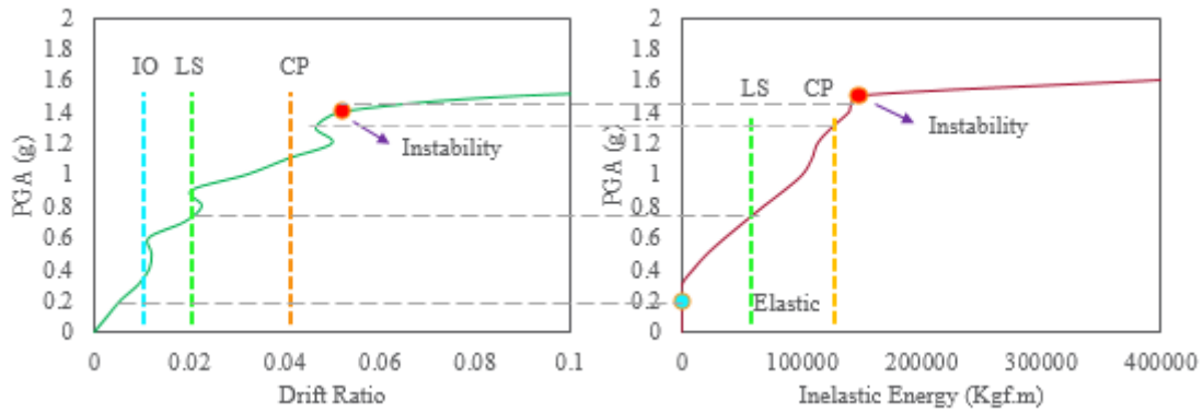
Fig.14. comparison of IDA curve under Imperial Valley record in ten-story building with drift and energy methods
