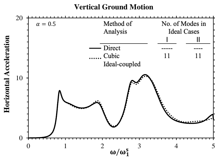
(c) Cubic ideal-coupled method
