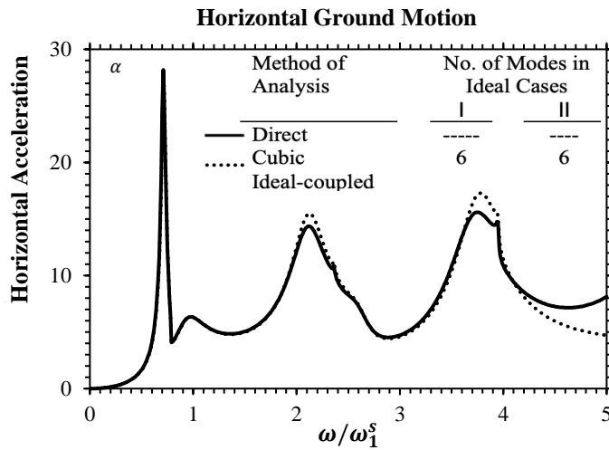
(c) Cubic ideal-coupled method
