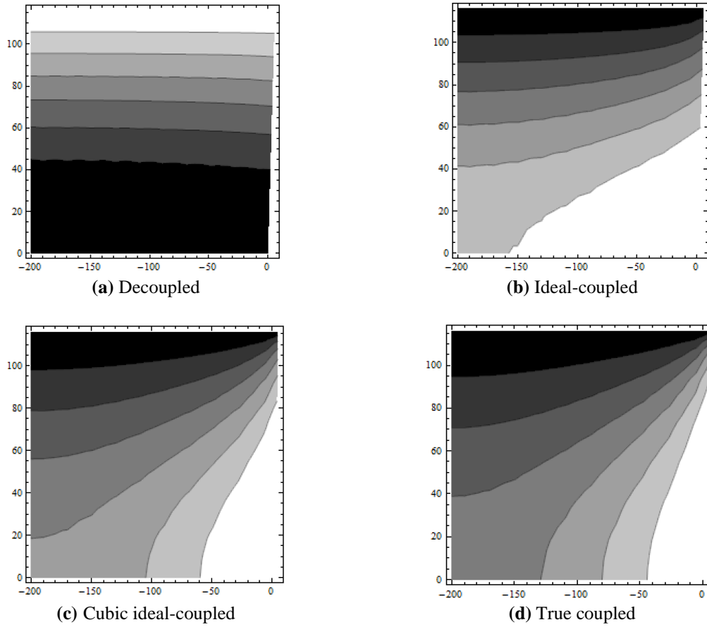
Fig. 11. First pressure mode shapes
