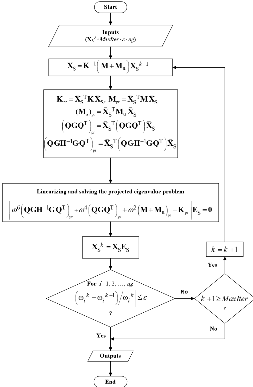
Fig. 1. Flowchart of generalized subspace method for Eigenproblem (16)
