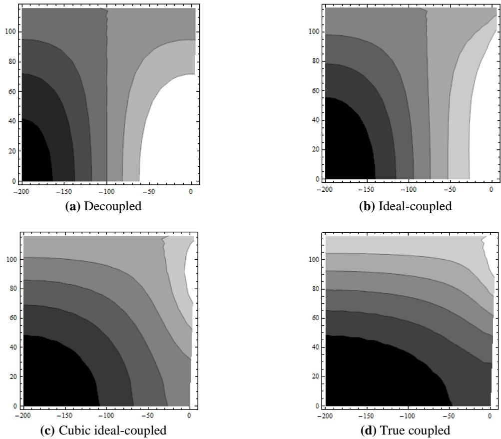
Fig. 12. Second pressure mode shapes
