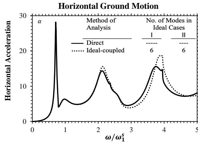
(b) Ideal-coupled method
