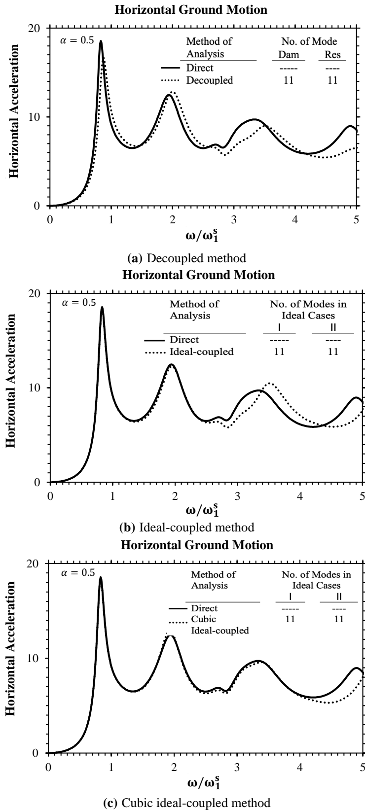
Fig. 17. Frequency response function at the dam crest resulting from horizontal excitation with \alpha = 0.5
