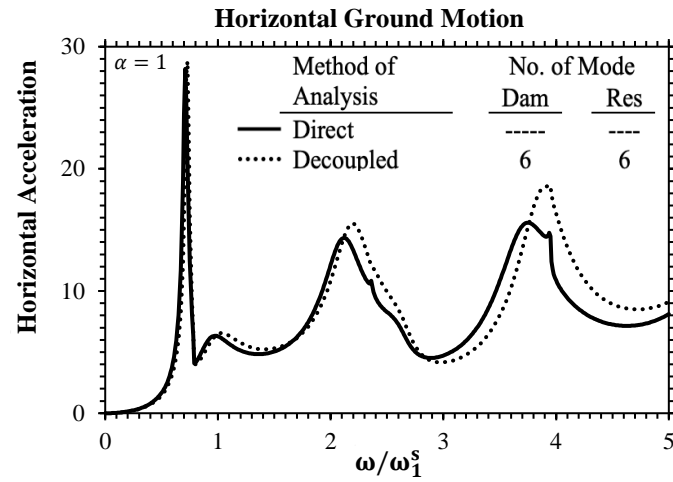
(a) Decoupled method
