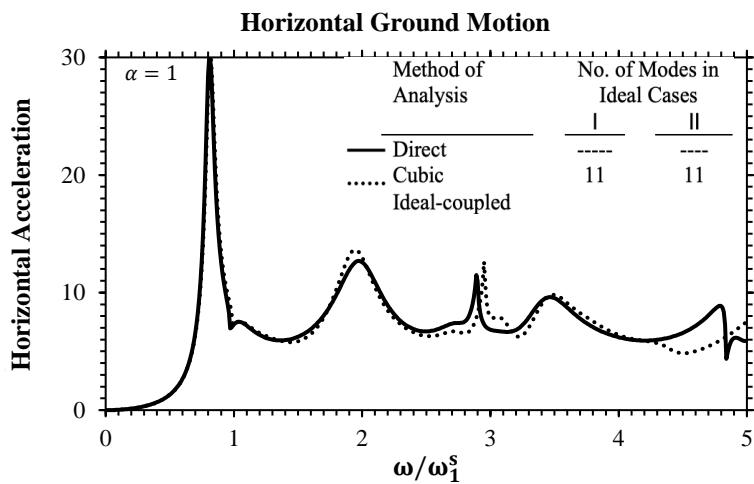
(c) Cubic ideal-coupled method
