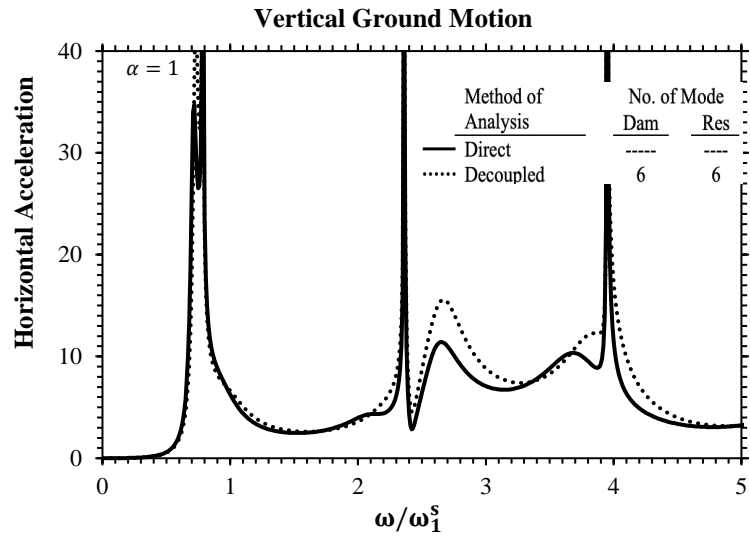
(a) Decoupled method
