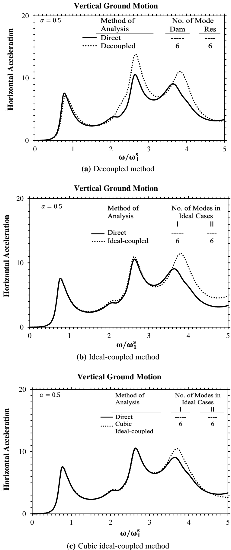
Fig. 8. Frequency response function at the dam crest resulting from vertical excitation with \alpha = 0.5
