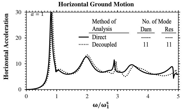
(a) Decoupled method
