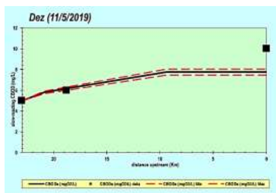
Fig 13. Simulation of BOD 5 in Dez River November 2019
