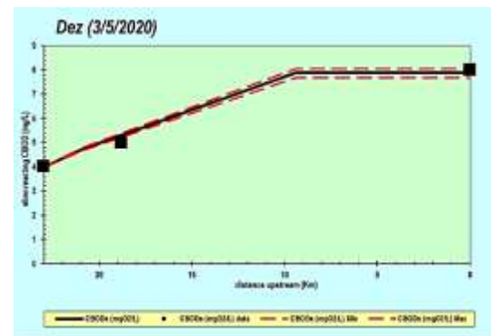
Fig 17. Simulation of BOD 5 in Dez River March 2020
