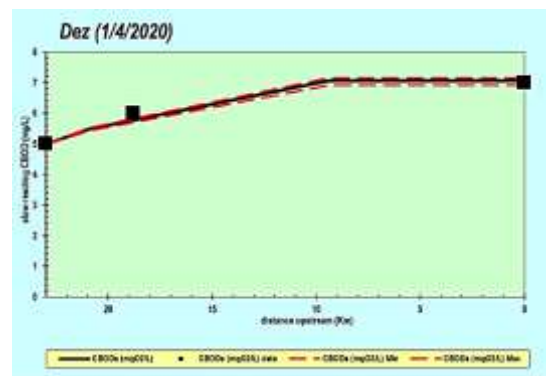
Fig 15. Simulation of BOD 5 in Dez River January 2020
