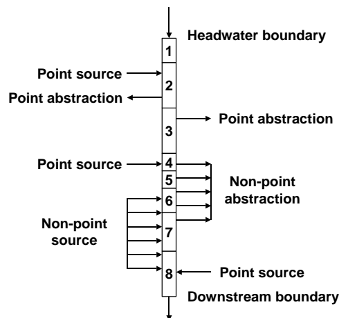
Fig 4. QUAL2Kw model subdivision for river without branches
