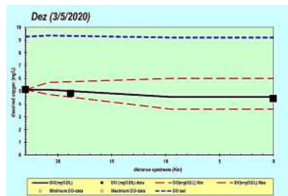
Fig 11. Simulation of DO in Dez River March 2020
