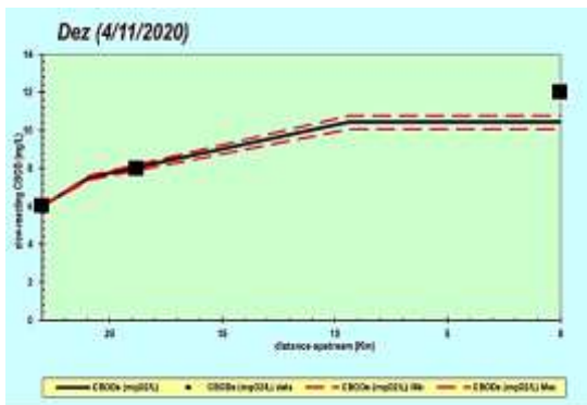
Fig 18. Simulation of BOD 5 in Dez River April 2020
