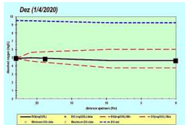
Fig 9. Simulation of DO in Dez River January 2020
