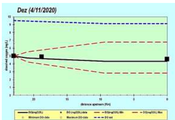
Fig 12. Simulation of DO in Dez River April 2020
