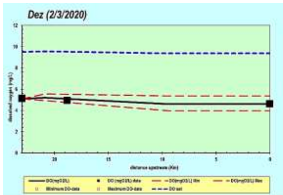
Fig 10. Simulation of DO in Dez River February 2020
