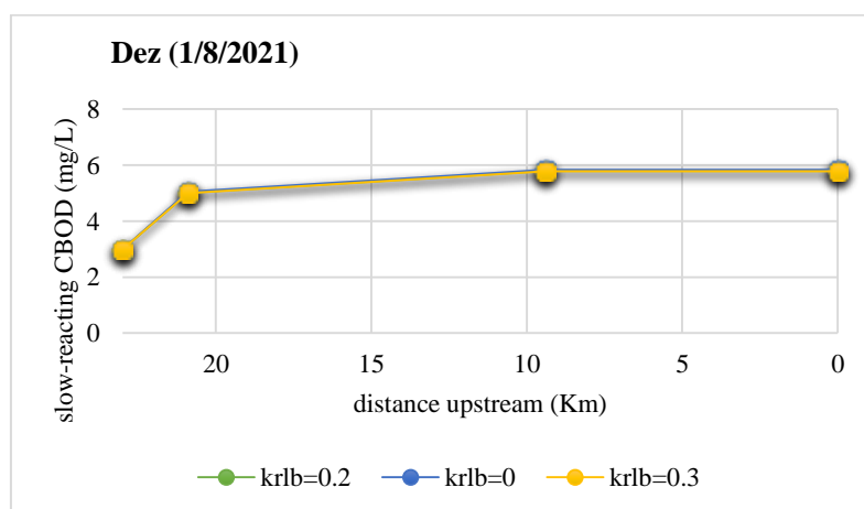
Fig 21. Investigation of changes in BOD simulation changes by changing the basal rate of algal respiration
