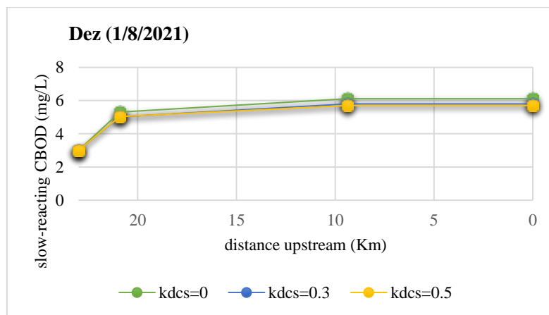
Fig 20. Investigation of changes in BOD simulation by changing the value of BOD oxidation rate
