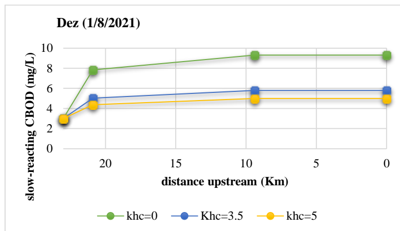
Fig 19. Investigation of changes in BOD simulation by changing the value of BOD hydrolysis rate
