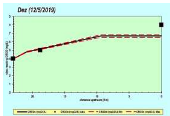
Fig 14. Simulation of BOD 5 in Dez River December 2019
