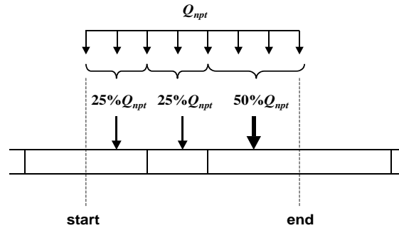
Fig 6. Way of considering non-point input sources to an element in the QUAL2Kw
