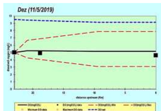
Fig 7. Simulation of DO in Dez River November 2019
