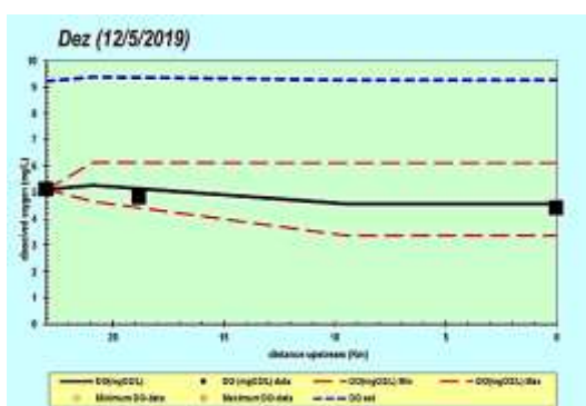
Fig 8. Simulation of DO in Dez River December 2019
