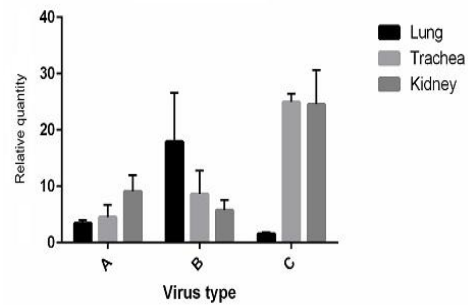
Figure 3. Comparison of relative viral quantity in lung, trachea and kidney between groups of chicken infected with different type of IBV (A, B and C).
