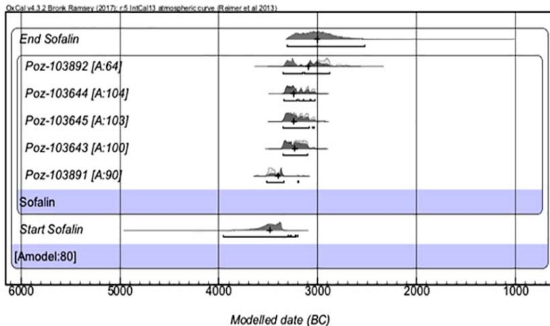
Figure 7: Modeled dates from Tappeh Sofalin (modeling using OxCal 4.3)
