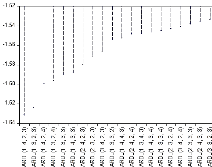
Figure 1: Akaike Information Criteria (Top 20 Models)
