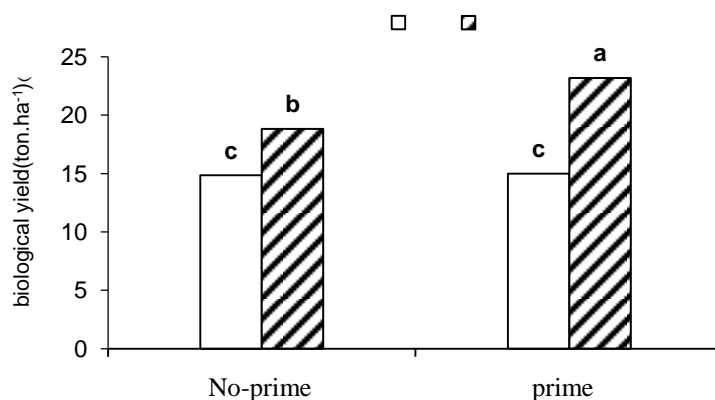
Figure 1. Comparison of the interactions of seed pre-treatment with salicylic acid and mycorrhizal fungi for biomass yield
