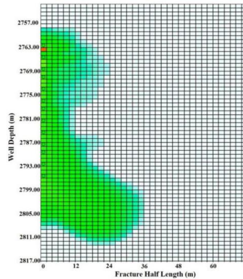
Figure 4. Fracture geometry in FDM model
