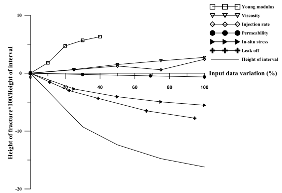
Figure 8. Effect of various parameters on the ratio of fracture height to interval height
