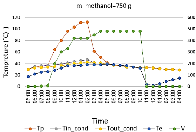
Fig. 8. The variation of generator, inlet and outlet condenser, evaporator temperatures and methanol concentration with time
