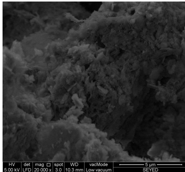
Fig. 9. Cementation crystals of the stabilized soil specimen with 18% OPC, 2% PA, and 5% SS after 24 h
