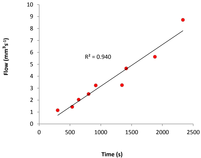
Fig. 4. Flow-time relationship of the untreated clay
