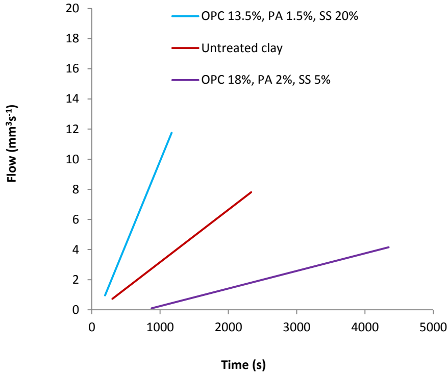
Fig. 6. Flow-time relationships of untreated and stabilized clay
