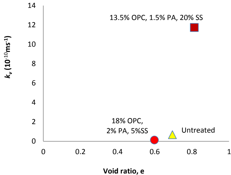
Fig. 7. Permeability-void ratio relationships under 1D consolidation tests
