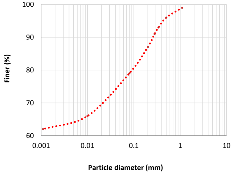
Fig. 2. Particle size distribution curve of the soil (Mousavi and Wong, 2015)
