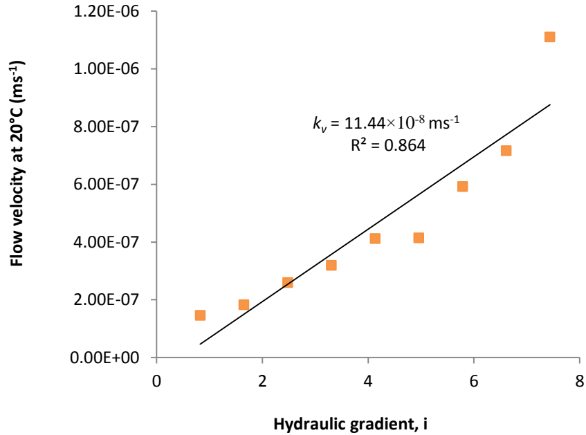
Fig. 3. Rate of permeability of the untreated clay
