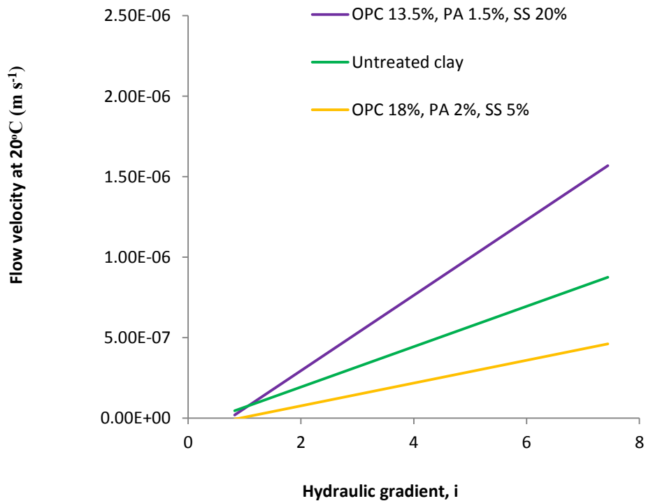
Fig. 5. Rate of permeability of the untreated and stabilized soil specimens
