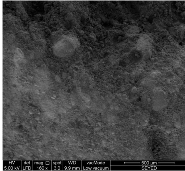
Fig. 8. SEM micrographs taken from the surface of the stabilized soil specimen with a binder composition of 18% OPC, 2% PA, and 5% SS (Mousavi and Wong, 2015)
