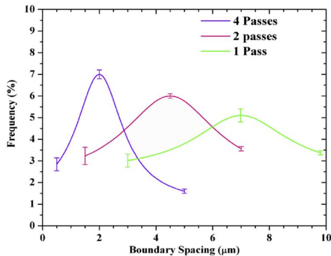
Fig. 7. Boundary spacing histogram in AZ31 alloy deformed to various number of ABE passes [53]
