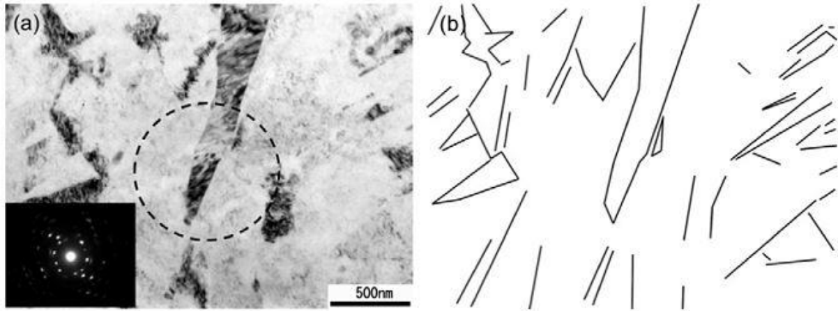
Fig.5. Microstructure of a multipass MDFed sample. The twin boundaries visible in (a) are identified more precisely in (b) [24]
