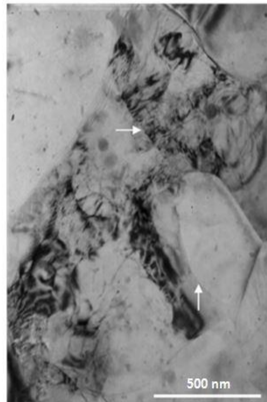
Fig. 4. Representative TEM micrographs of AZ31 after ECAP, showing the presence of subgrain structures [62]
