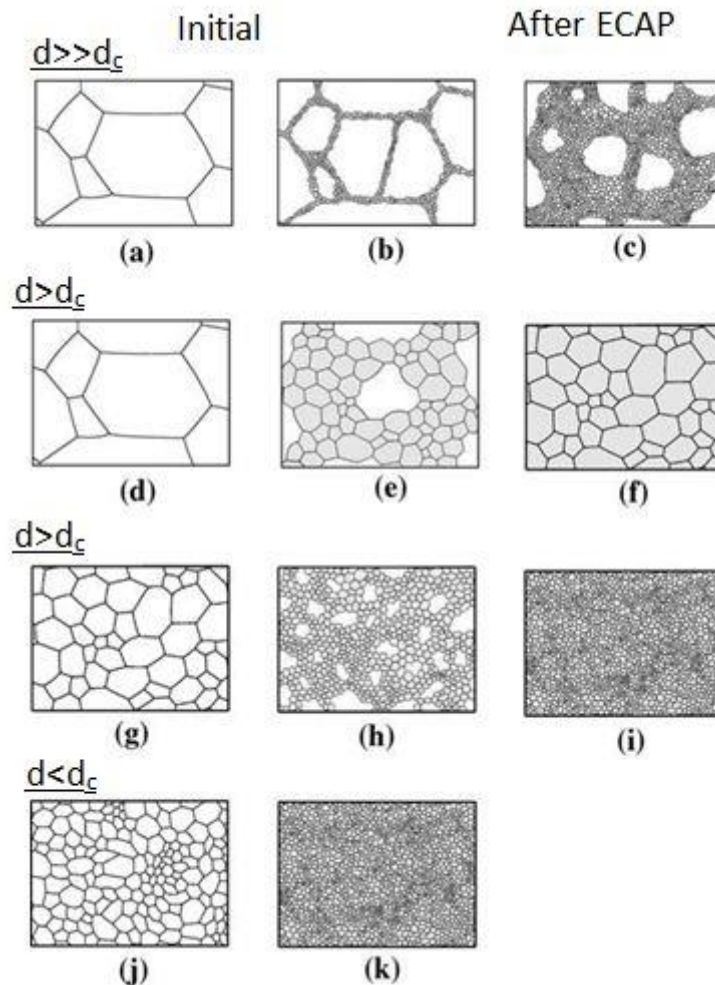
Fig. 2. A model for the grain refinement of magnesium alloys processed by ECAP [6]
