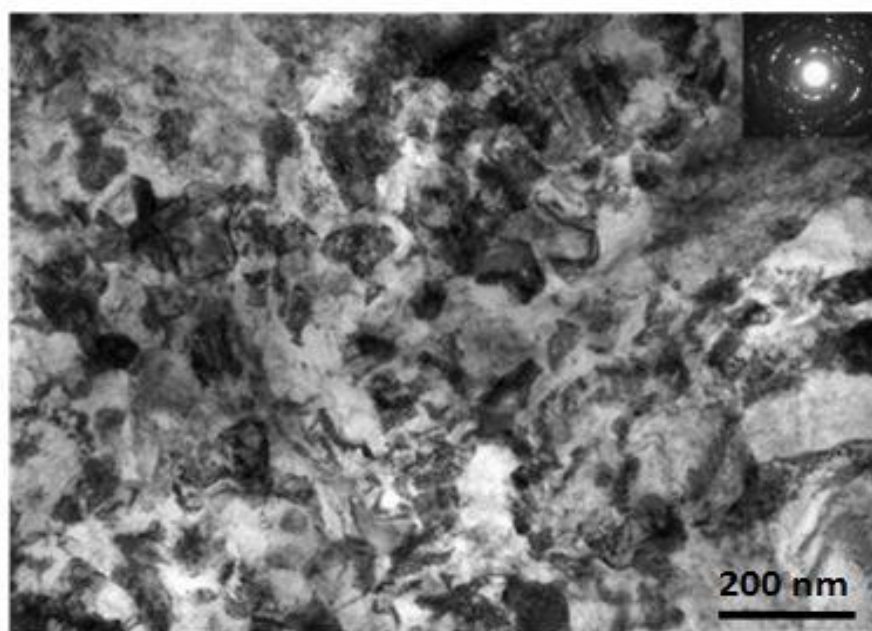
Fig. 1. Typical nano grains developed after single pass ABE
