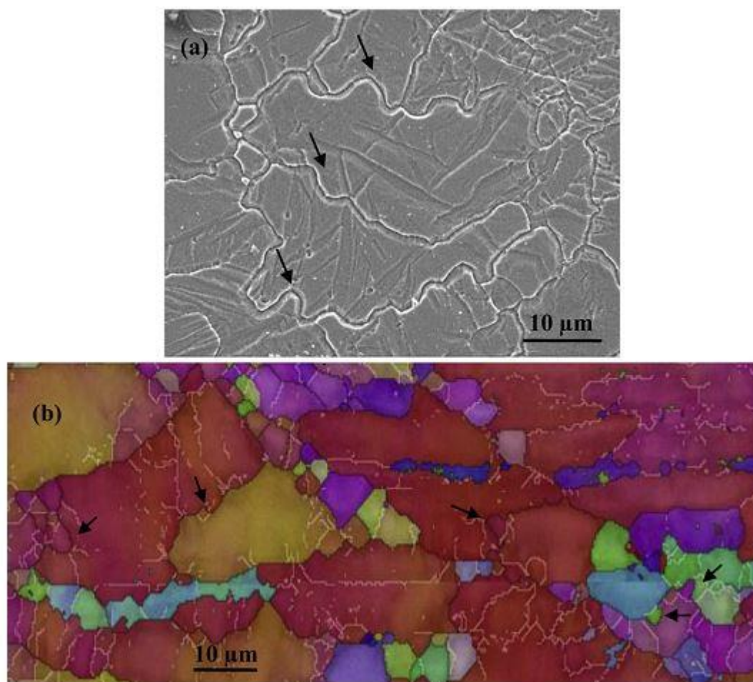
Fig. 3. a) and b) The microstructure of AZ31 alloy deformed to the first step of ABE process showing the bulging of GBs [53]
