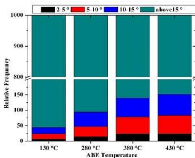
Fig. 8. The distribution of boundary misorientation in AZ31 alloy after single pass ABE at different temperature
