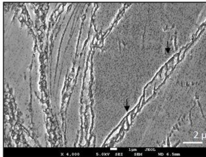
Fig. 6. Recrystallized grains within twin during in an ABE AZ31 alloy
