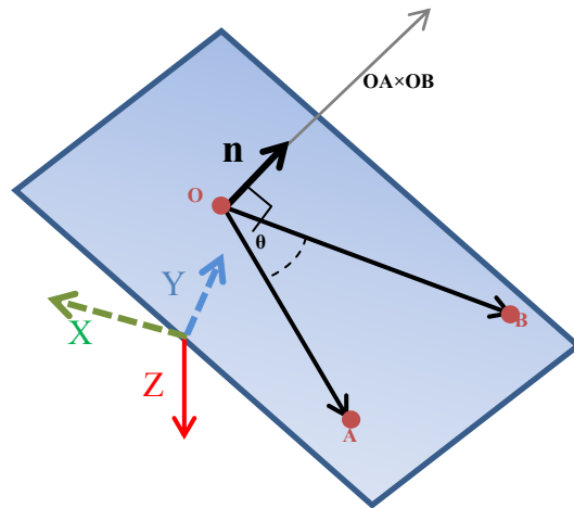
Figure 4: Finding the unit normal vector of the surface
