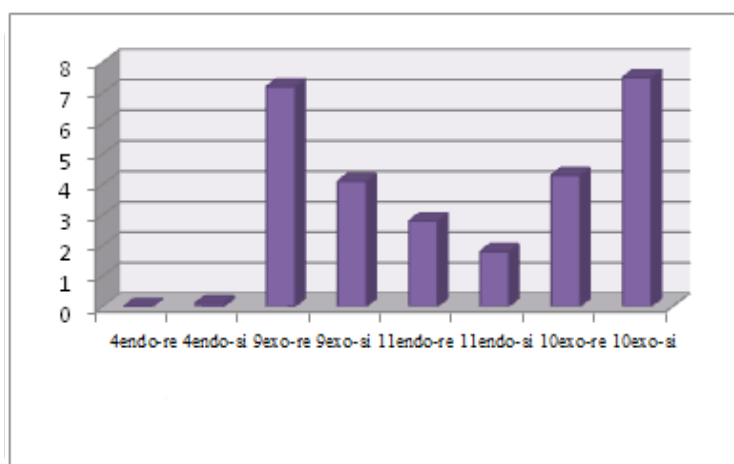
Figure 3. Relative energy of possible transition structures
