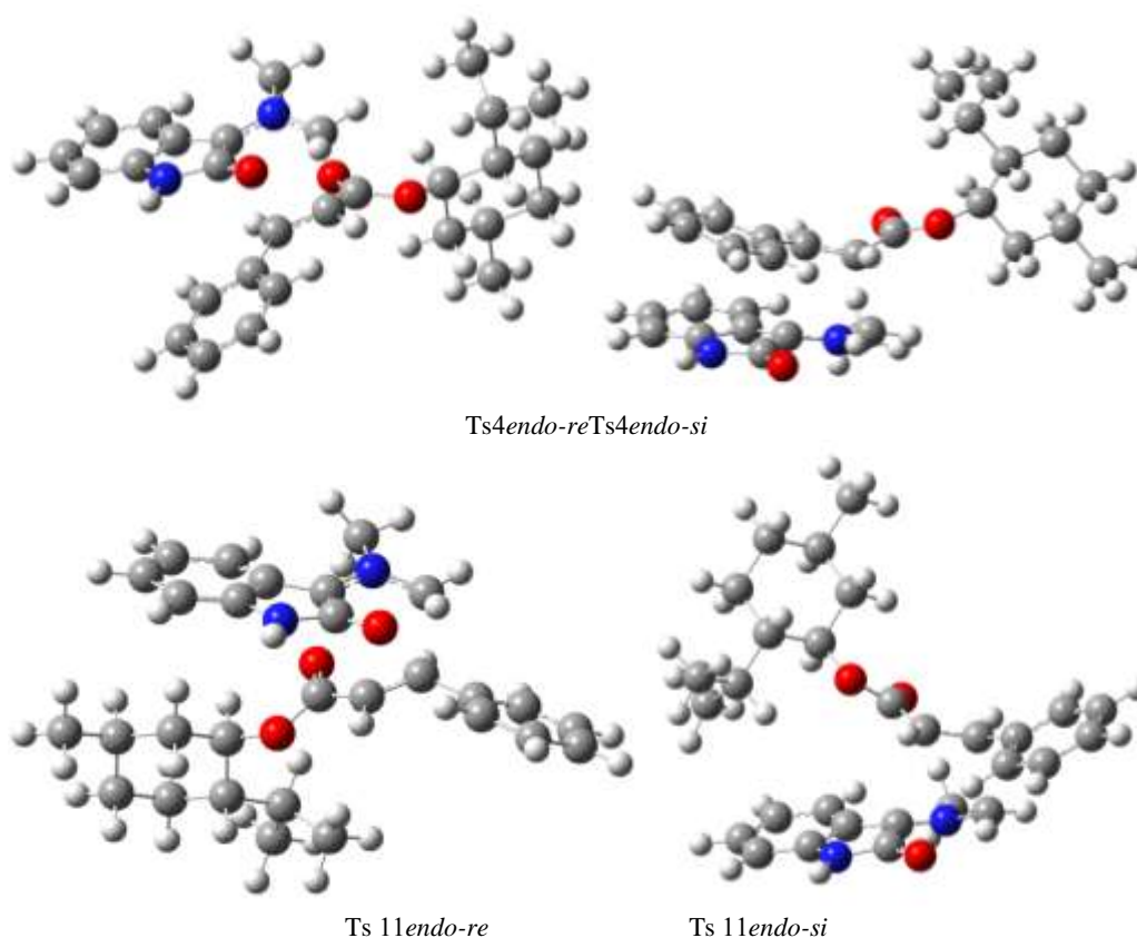
Figure 2. Selected optimized transition structures at the B3LYP/6-311G(d,p) corresponding to the regiosomeric path of the 1,3-dipolar cycloaddition reaction 5 and 7.
