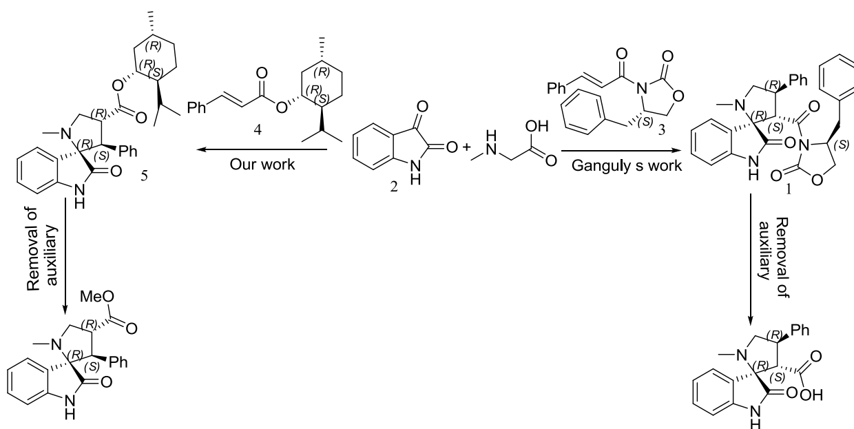
Scheme 1. Synthesis of chiral spirooxindolopyrrolidines 1, 5
