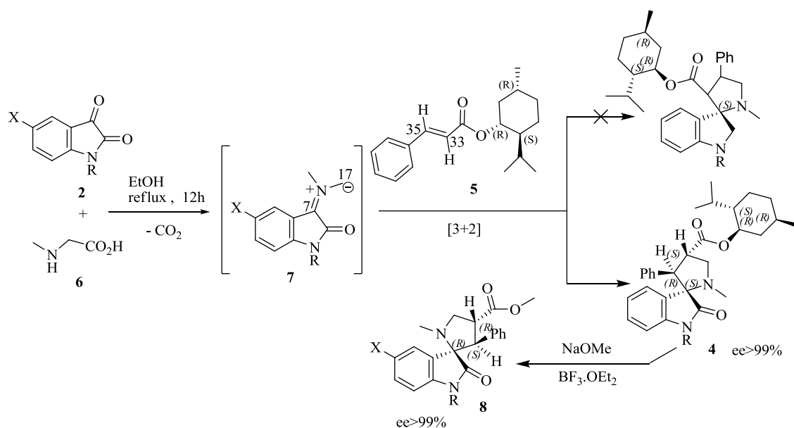
Scheme 2. Synthesis of chiral spirooxindolopyrrolizidines 4, 8
