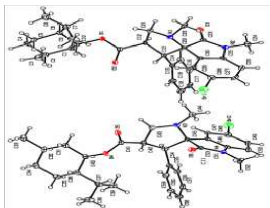
Figure 1. The ORTEP diagram of one of the two crystallographic independent molecules in the asymmetric unit of 4g is shown. Thermal ellipsoids are at 30% probability level.
