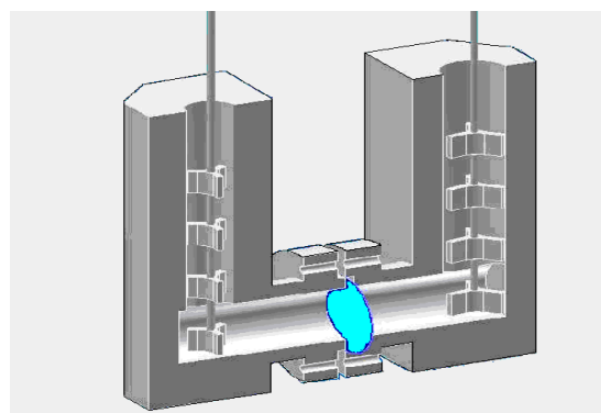
Fig. 2. Experiment Apparatus
