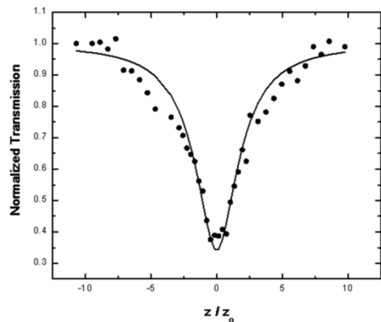
Figure 5. Shows open aperture Z-scan measurement of the silver nanoparticles dispersed in water. The solid curve is the theoretical fit for the nonlinear absorption process.
