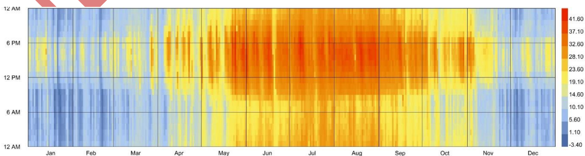
Chart 3. Dry bulb temperature of Gorgan, Iran, hourly temperature (°C), from January to December, in the period of 2009-2023 (Climate.onebuilding.org, 2018).
