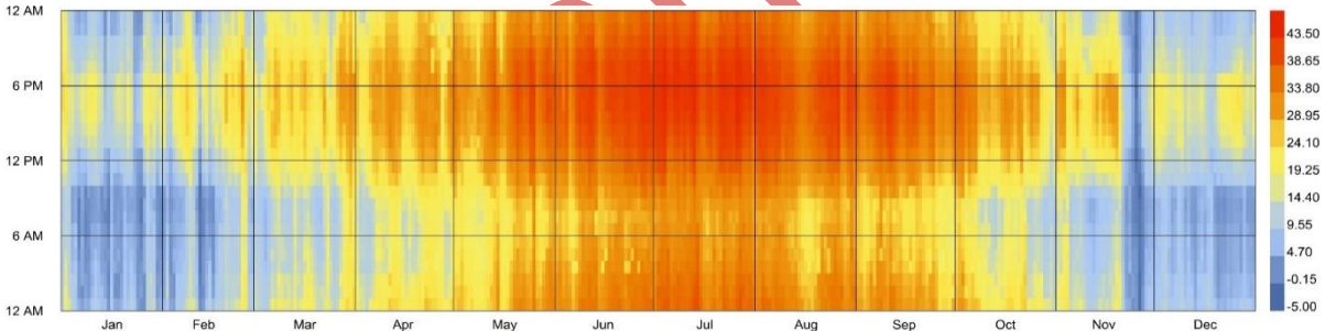
Chart 2. Dry bulb temperature of Yazd, Iran, hourly temperature (°C), from January to December, in the period of 2009-2023 (Climate.onebuilding.org, 2018).
