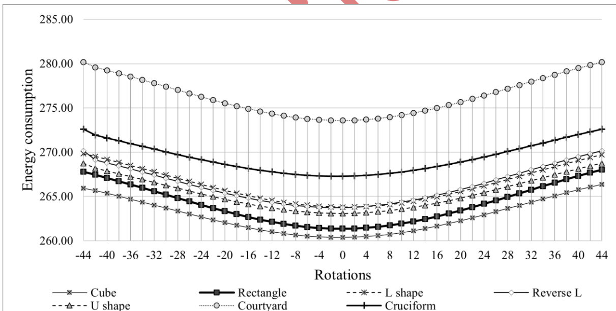
Chart 8. Energy consumption of selected forms for Shahrekord.
