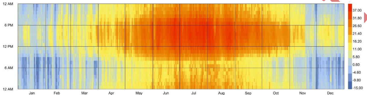
Chart 1. Dry bulb temperature of Shahrekord, Iran, hourly temperature (°C), from January to December, in the period of 2009-2023 (Climate.onebuilding.org, 2018).
