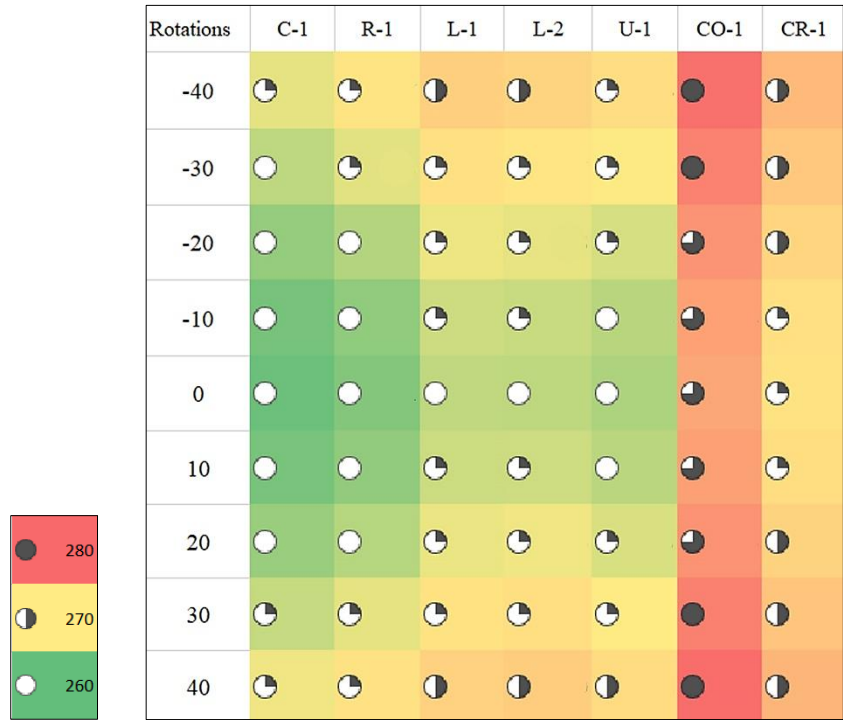
Figure 7. Heat Map of Annual Energy Consumption for Different Building Forms and Rotations in Shahrekord
