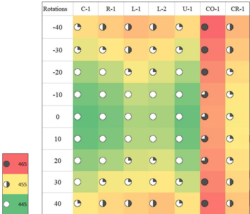
Figure 10. Heat Map of Annual Energy Consumption for Different Building Forms and Rotations in Qeshm
