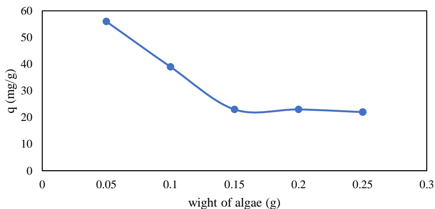
Fig. 3. Effects of the weight of algae on the RIF biosorption in C. sorokiniana MH923013 at an initial concentration of 100 ppm
