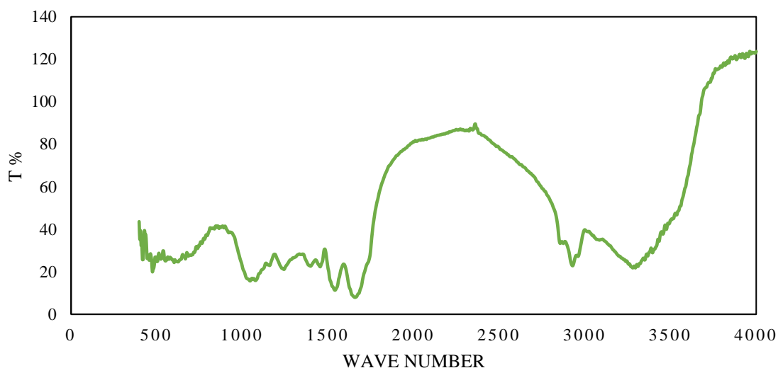
Fig. 8. FTIR for algae C. sorokiniana MH923013
