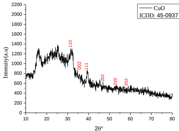
Figure 2 . XRD pattern of CuO nanoparticles
