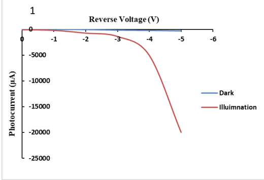
H :P–V curve for 7% Ag-doped hybrid junction
