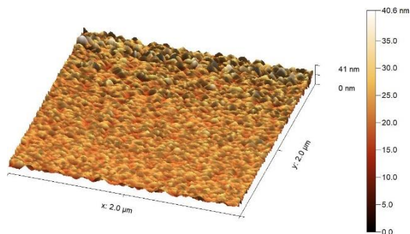
Figure 10. 3D AFM surface plot of Ag nanoparticles over a 2 \times 2 \mu\text{m}^2 scan area, showing grain peaks up to 40 nm in height
