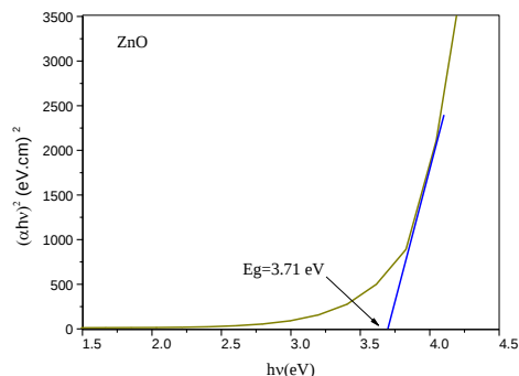
Figure 19. Tauc plot of ZnO thin film showing a band gap of 3.71 eV, reflecting nanocrystalline behavior and surface effects
