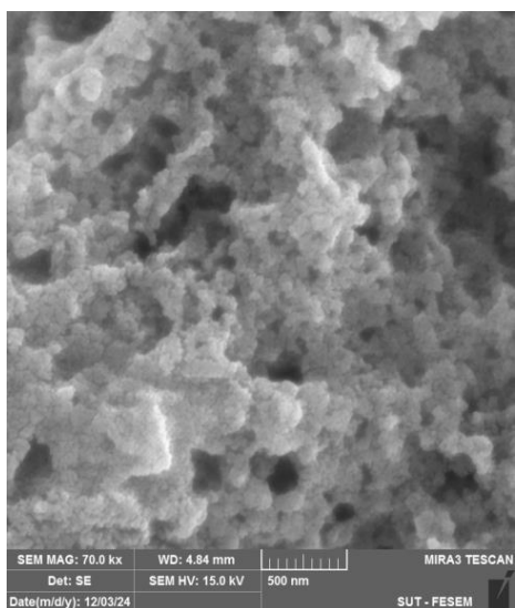
Figure 5. FE-SEM Images of CuO Nanoparticles
