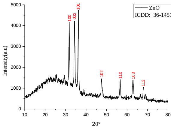
Figure 3. XRD pattern of ZnO nanoparticles
