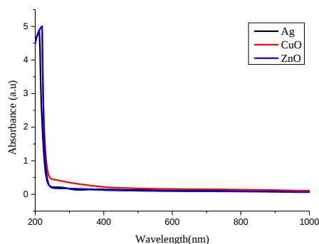
Figure 16. The experimental optical absorbance curve of silver nanoparticles (Ag – CuO and ZnO NPs)
