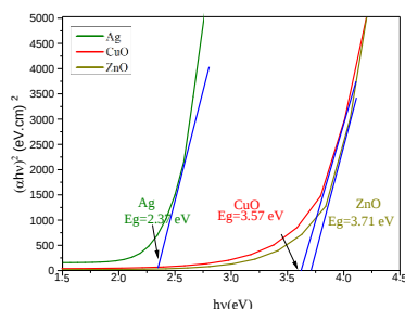
Figure 20. Combined Tauc plots of Ag, CuO, and ZnO films highlighting their enhanced optical band gaps
