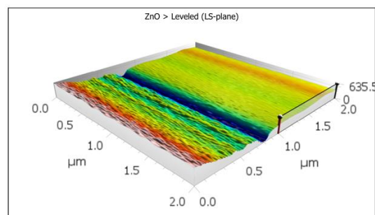
Figure 14. Leveled AFM Image (Z-Height up to ~635.5 nm)
