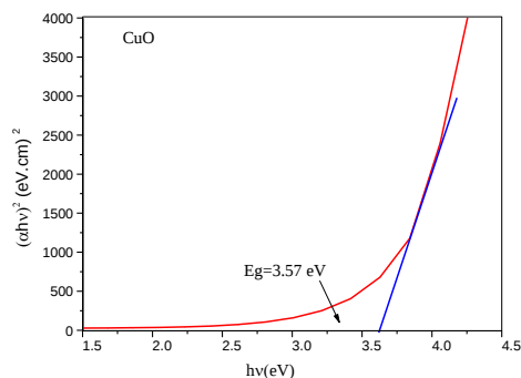
Figure 18. Tauc plot of CuO thin film indicating a band gap of 3.57 eV, attributed to quantum confinement effects.
