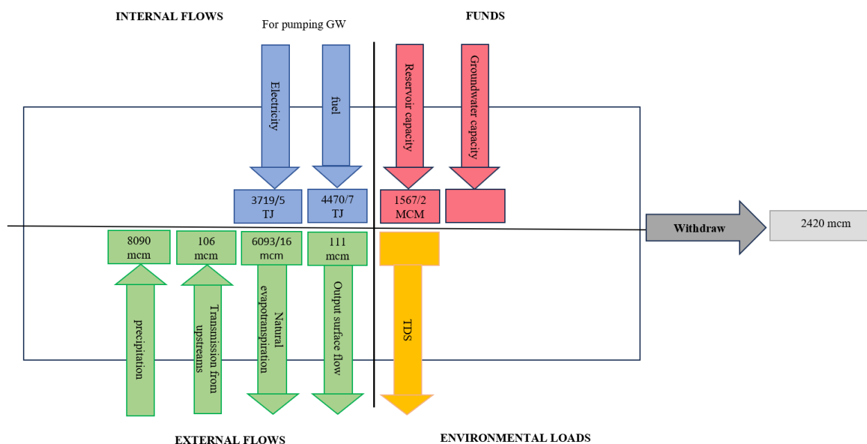
Figure4. Sized processor of the functional element local water withdraw(Iran)
