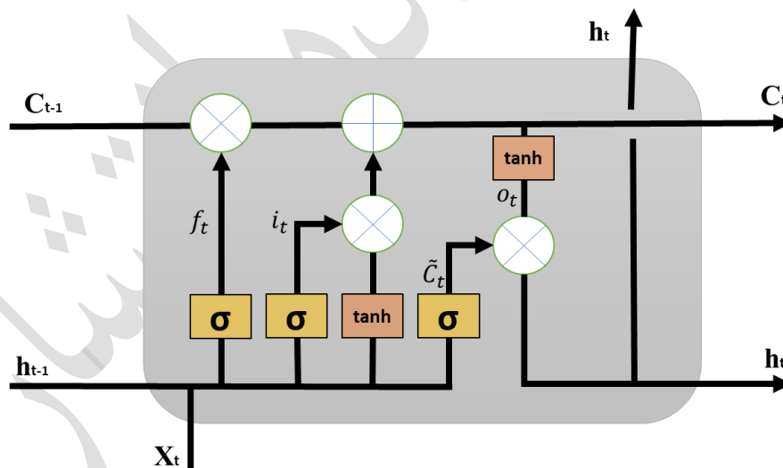
Figure 7. The internal structure of LSTM
